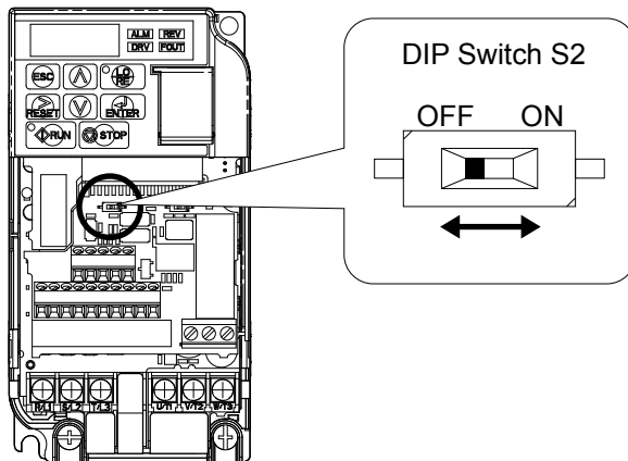
3.30 Interruptor DIP S2
