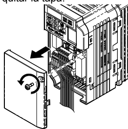
7.17 Quite la tapa
