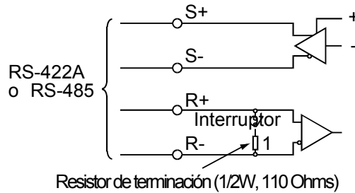
C.2 Interruptor MEMOBUS/Modbus
