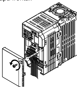
6.5 Quite la tapa frontal
