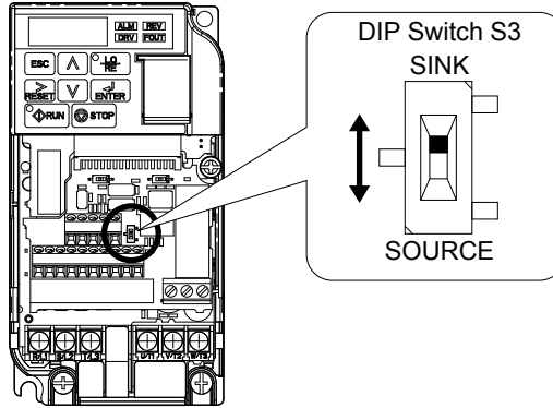
3.26 Interruptor DIP S3
