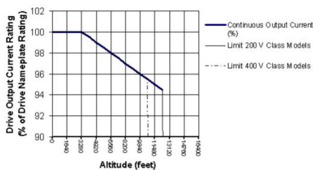
Altitude Derating for Yaskawa Inverters (feet)
