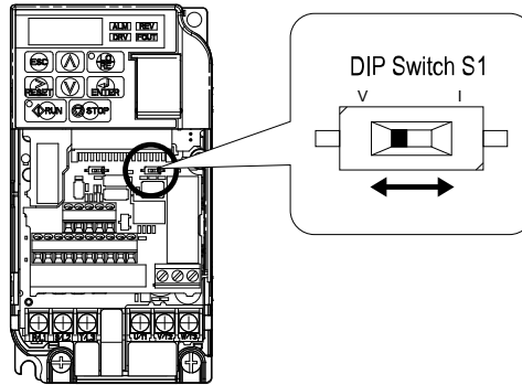
3.29 Interruptor DIP S1
